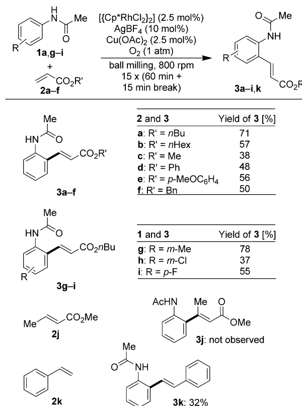
Scheme 2. Mechanochemical rhodium-catalyzed ortho -olefination of acetanilides. Bn = benzyl.
